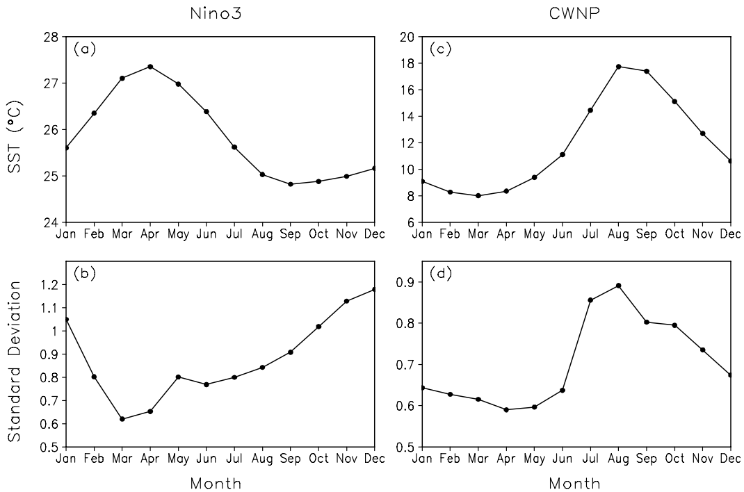
Fig. 5. Annual cycle of SST (upper panels) and standard deviation (bottom panels) for the Niño-3 region (left panels) and the CWINP region (right panels) as a function of calendar month.
