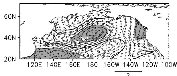
Fig. 8. Correlation between SSTAs in the CWNP region and geopotential height (contour) and wind (vector) anomalies at 850 hPa in the North Pacific during summer (July). The counter interval is 0.1, and shading indicates correlation coefficient values with 95% confidence level.
