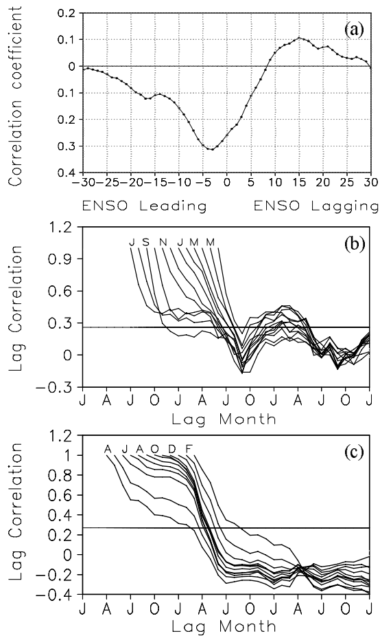
Fig. 12. (a) Monthly lead-lag correlation between SSTAs in the CWP region and the Niño-3 region. Negative lags refer to SSTAs in the Niño-3 region leading those in CWP. (b) Lag correlation of SSTAs in the CWP region, but with the ENSO-regressed SSTAs subtracted from the original data. (c) Same as panel (b), but for the ENSO-regressed SSTAs.
